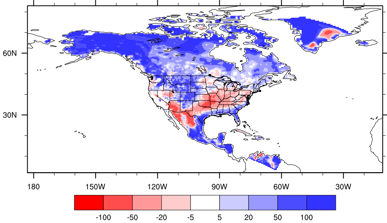
lake_25_001 precipitation bias versus UDEL, Sep percent
