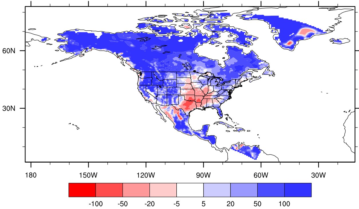
lake_25_001 precipitation bias versus UDEL, Oct percent
