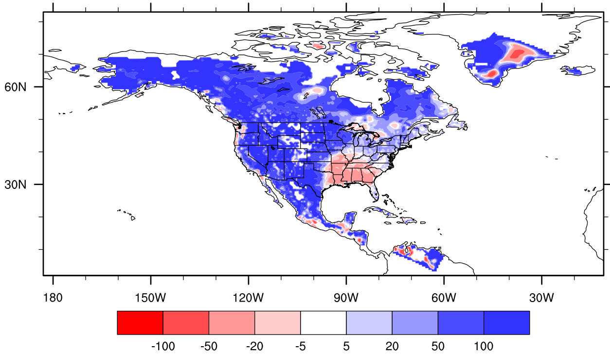
lake_25_001 precipitation bias versus UDEL, Jan percent
