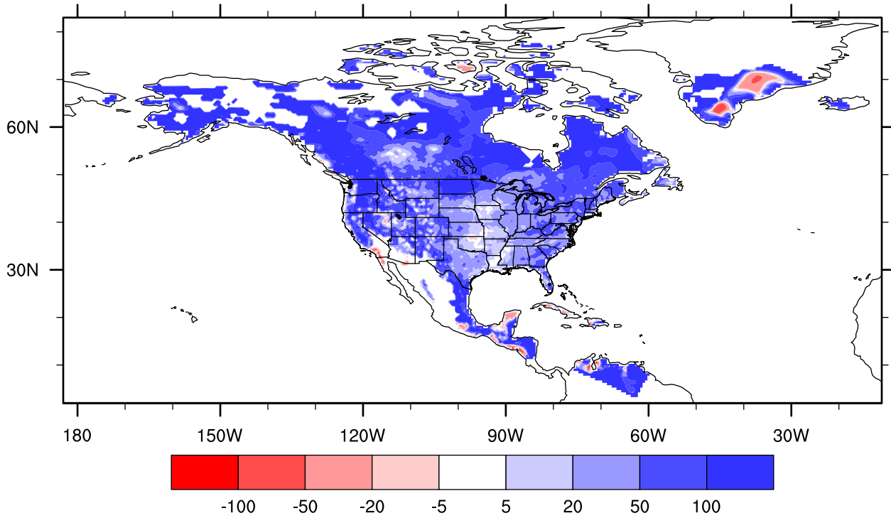
lake_25_001 precipitation bias versus UDEL, Apr percent
