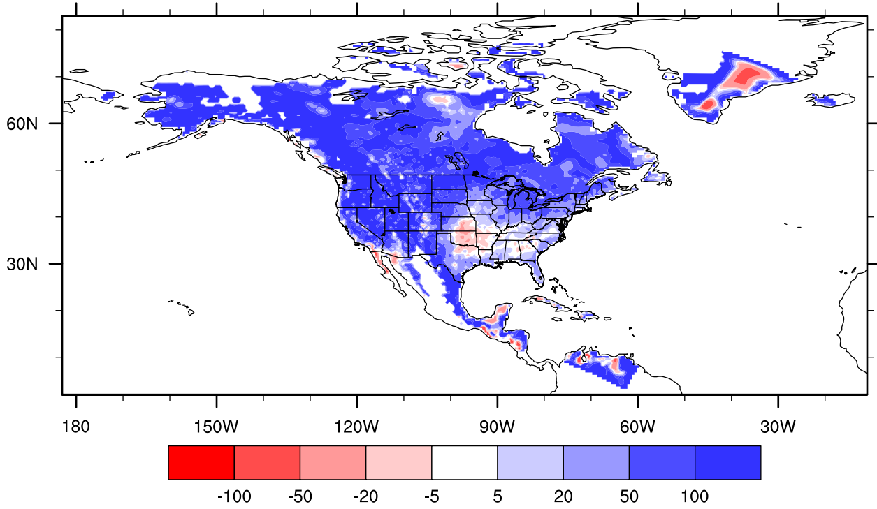
lake_25_001 precipitation bias versus UDEL, Mar percent
