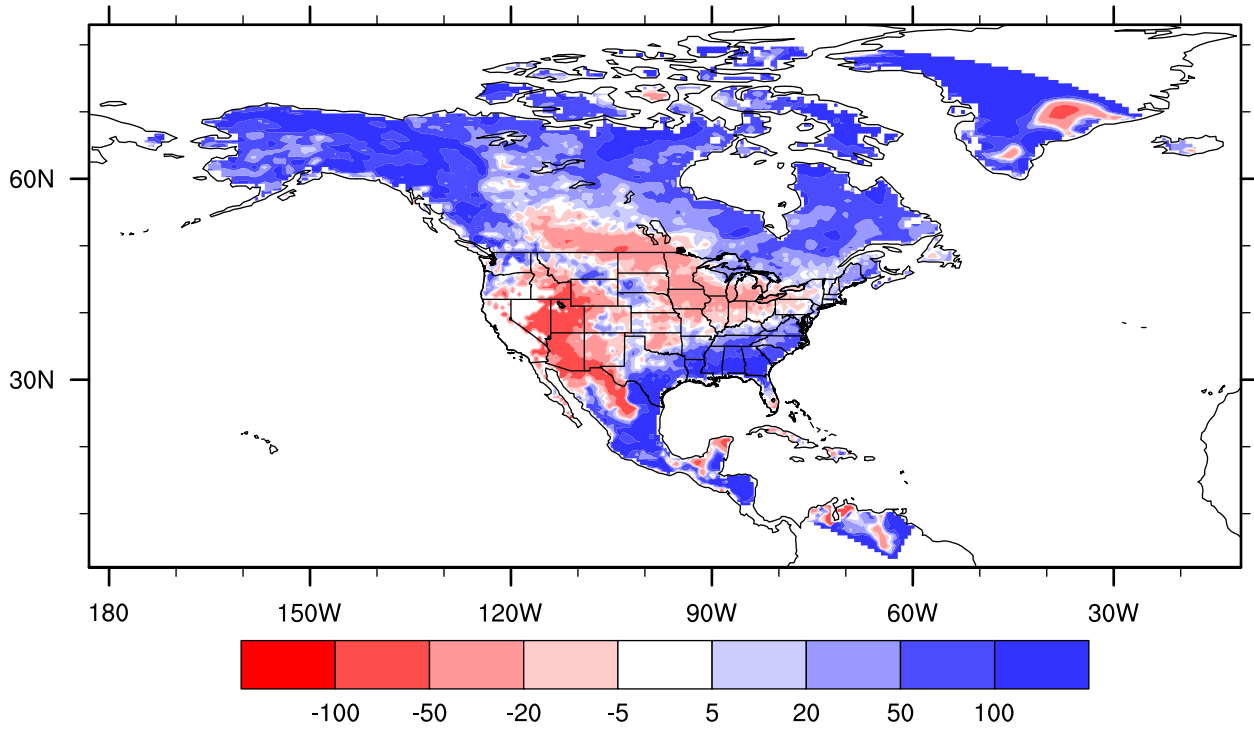
lake_25_001 precipitation bias versus UDEL, Aug percent
