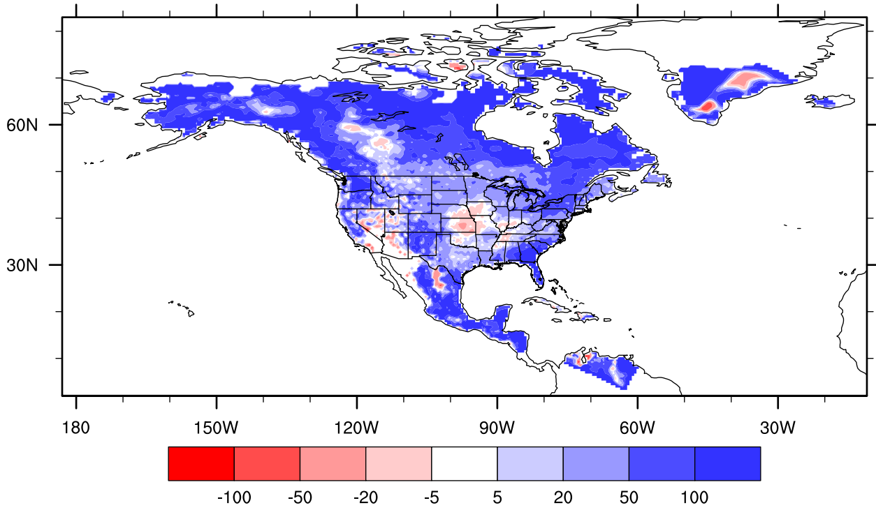
lake_25_001 precipitation bias versus UDEL, May percent
