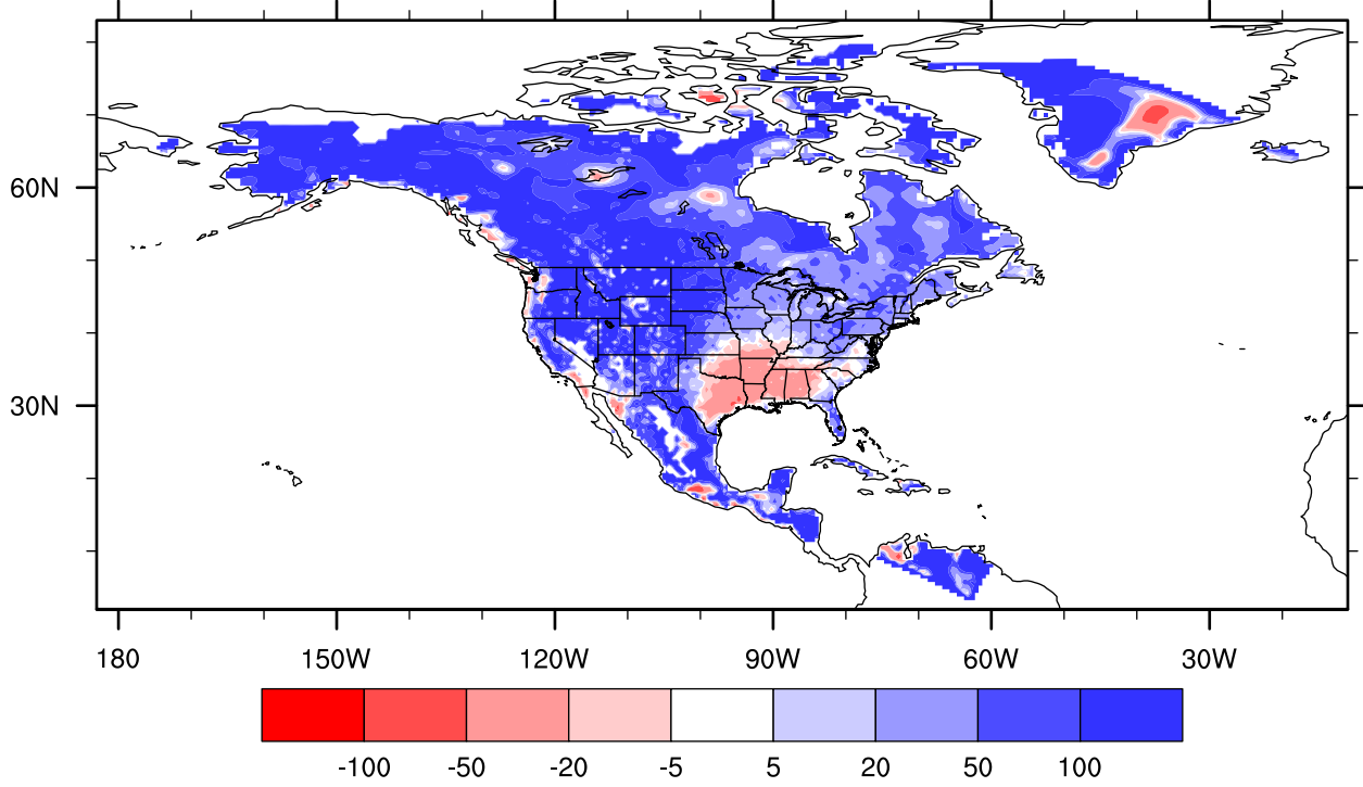
lake_25_001 precipitation bias versus UDEL, Nov percent
