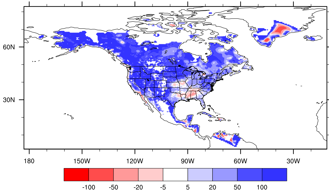
lake_25_001 precipitation bias versus UDEL, Feb percent
