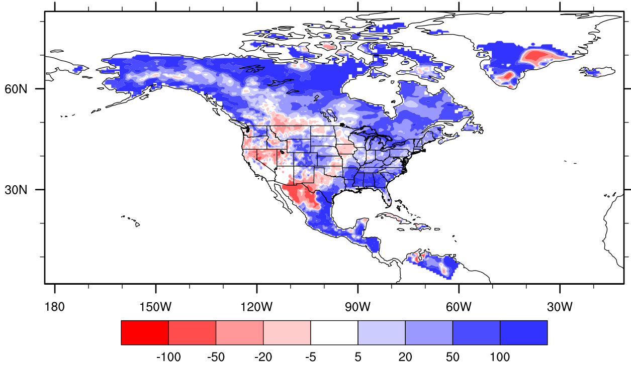
lake_25_001 precipitation bias versus UDEL, Jun percent
