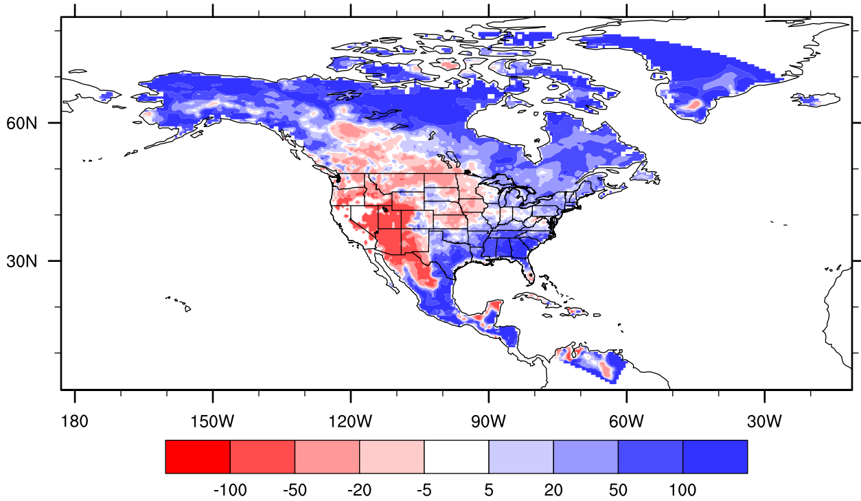
lake_25_001 precipitation bias versus UDEL, Jul percent
