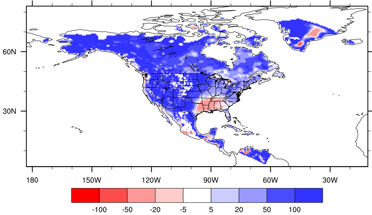
lake_25_001 precipitation bias versus UDEL, Dec percent
