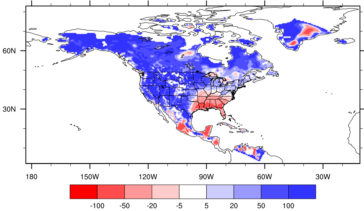
lake_25_003 precipitation bias versus UDEL, Jan percent
