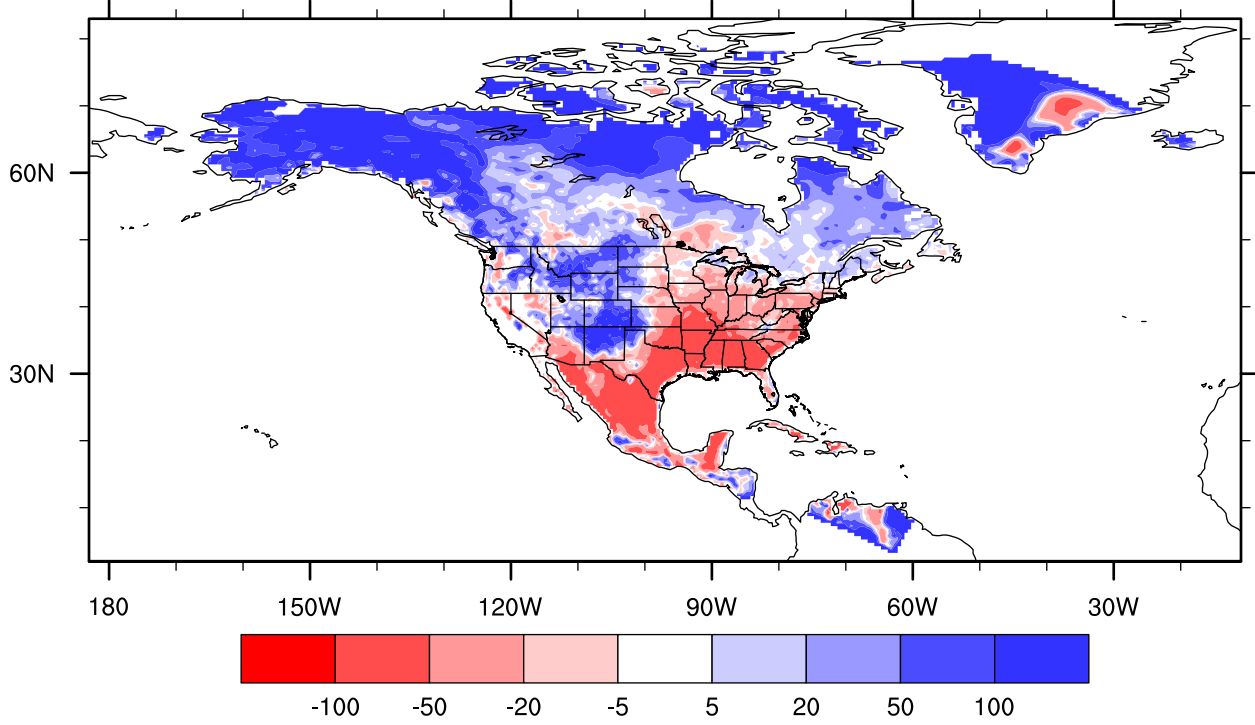
lake_25_003 precipitation bias versus UDEL, Sep percent
