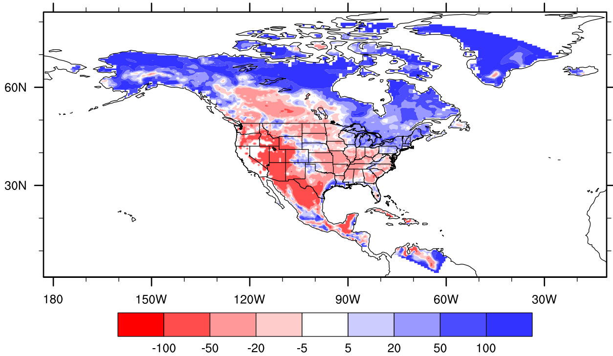
lake_25_003 precipitation bias versus UDEL, Jul percent
