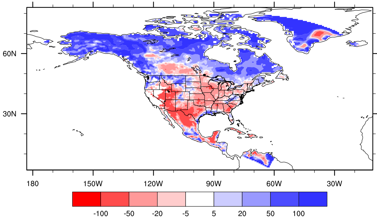
lake_25_003 precipitation bias versus UDEL, Aug percent
