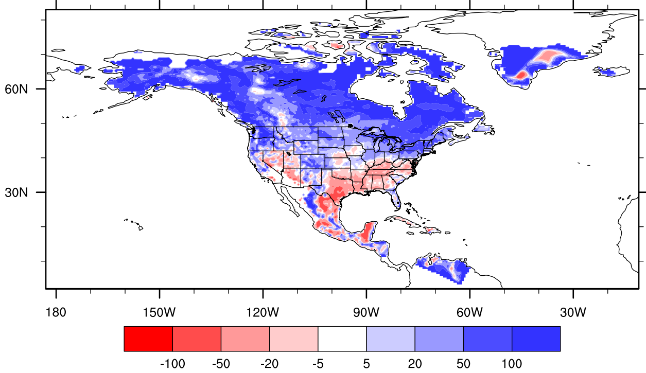
lake_25_003 precipitation bias versus UDEL, May percent
