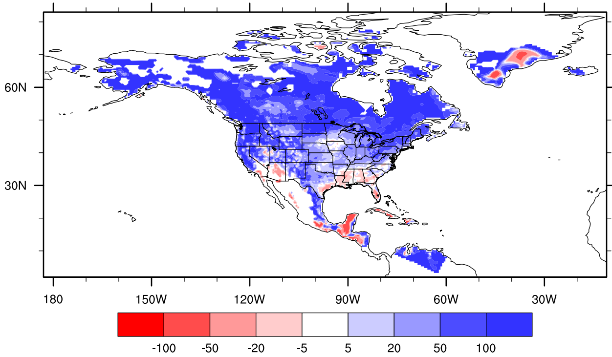
lake_25_003 precipitation bias versus UDEL, Apr
