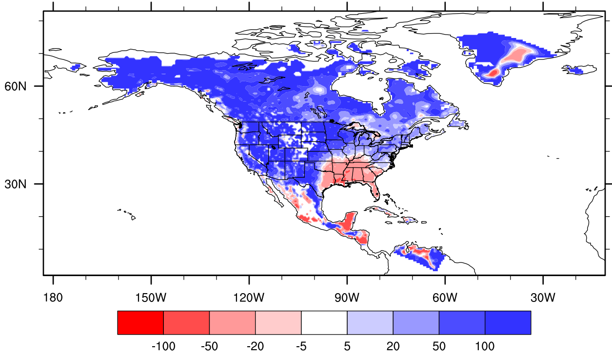
lake_25_003 precipitation bias versus UDEL, Dec percent
