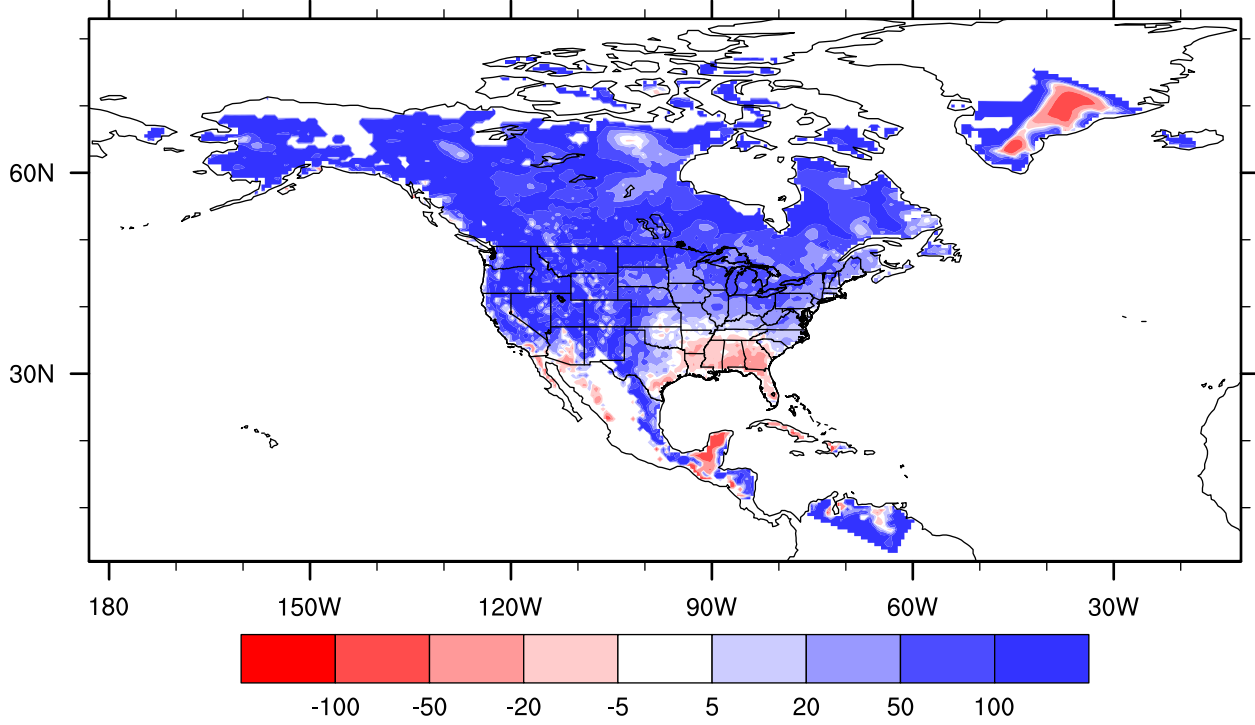
lake_25_003 precipitation bias versus UDEL, Mar percent
