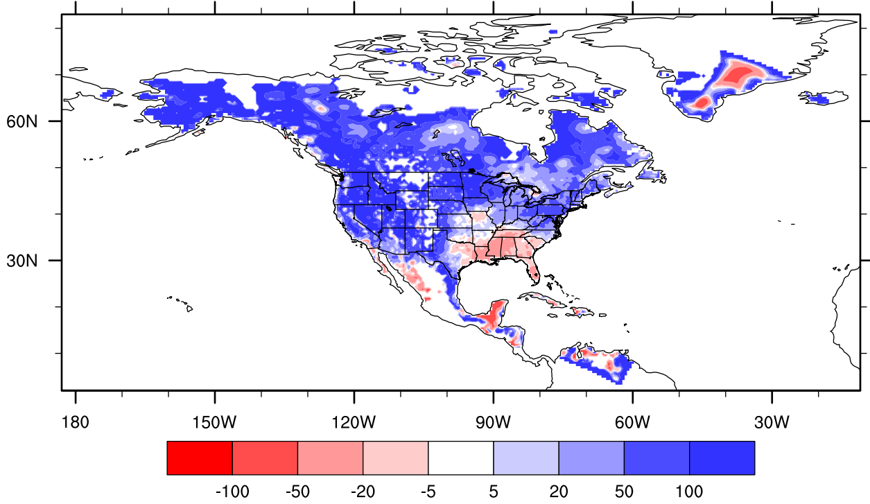
lake_25_003 precipitation bias versus UDEL, Feb percent
