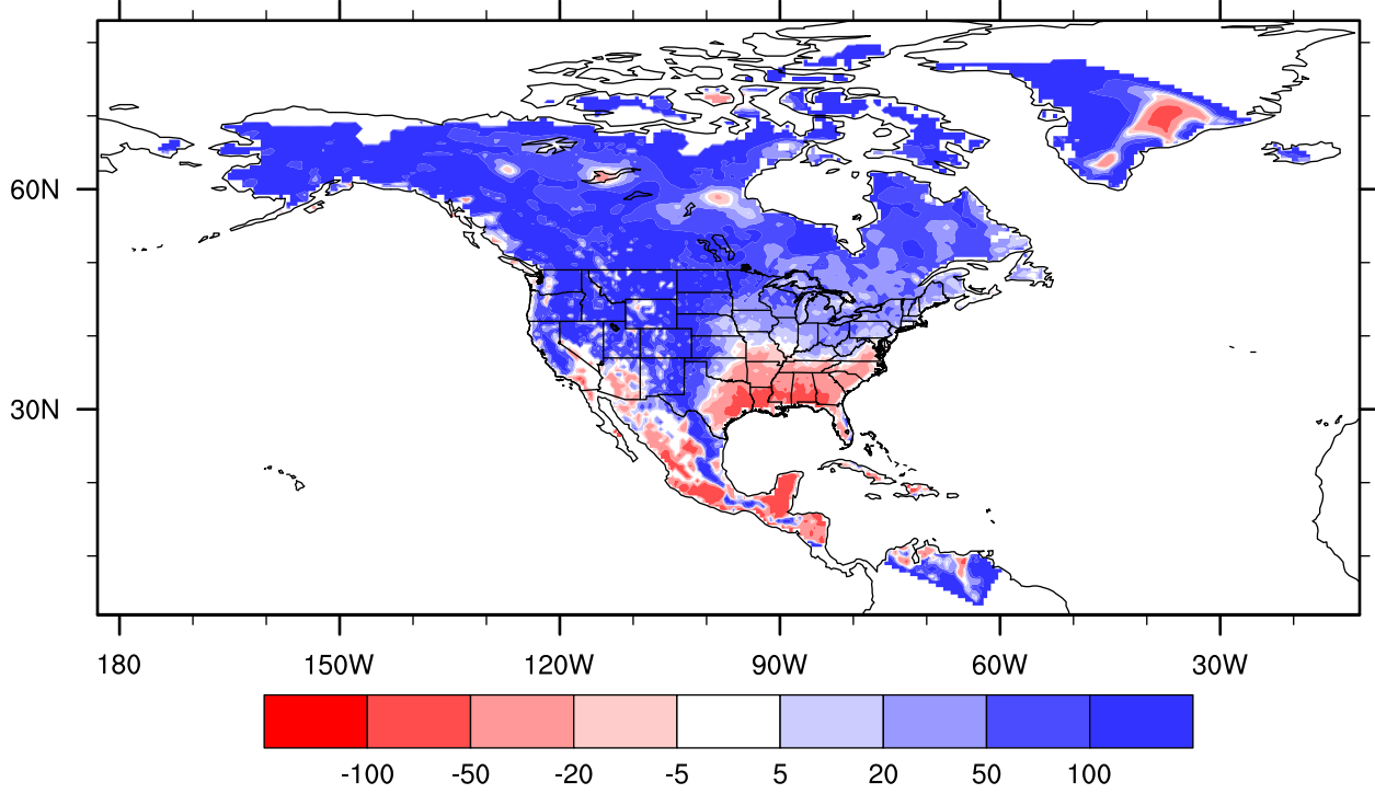
lake_25_003 precipitation bias versus UDEL, Nov percent
