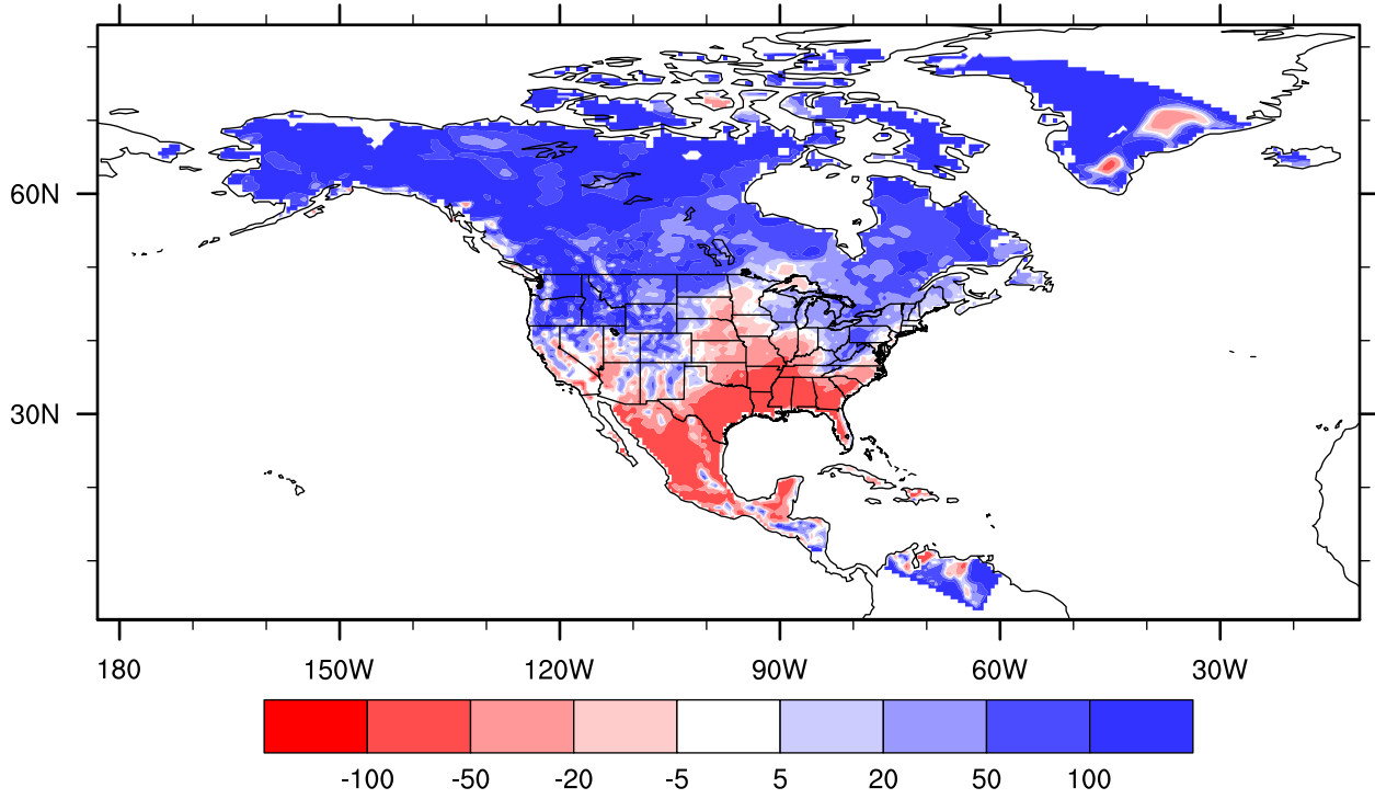
lake_25_003 precipitation bias versus UDEL, Oct percent
