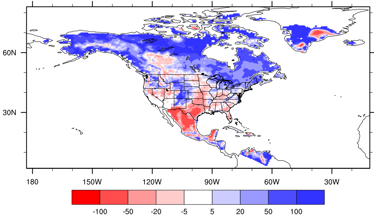
lake_25_003 precipitation bias versus UDEL, Jun percent
